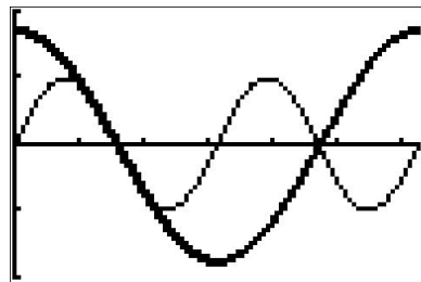
y = \sin(2x) and y = \sqrt{3}\cos(x)
