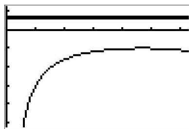
y = \frac{1}{\sin\left(\frac{1}{3}x - \pi\right)} and y = \sqrt{2}
