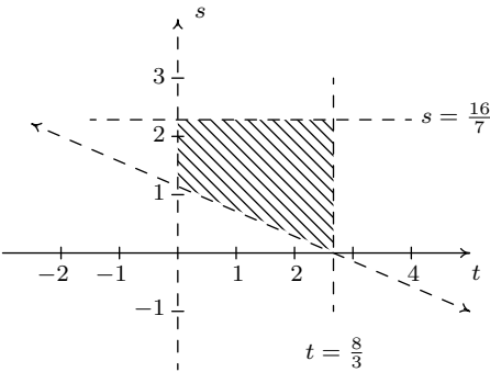
The region for our parameters s and t .
