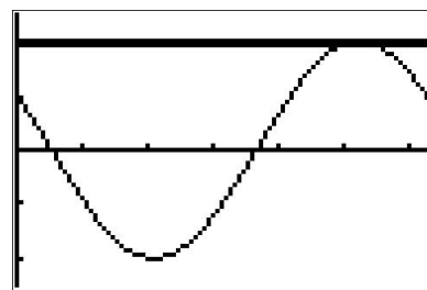
y = \cos(x) - \sqrt{3}\sin(x) and y = 2
